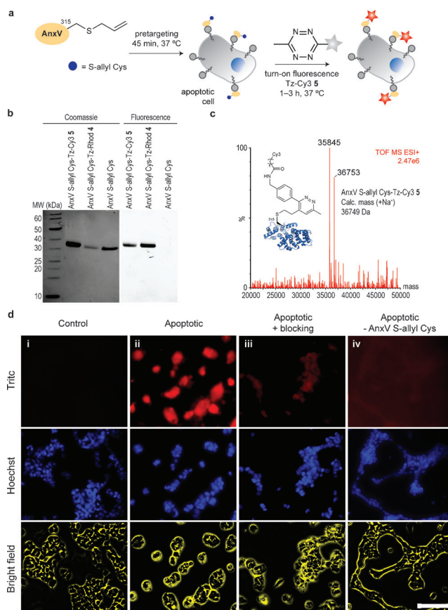
Figure 3. a) Pre-targeting of apoptotic cells with AnxV S-allyl Cys followed by IEDDA labeling with fluorogenic Tz-Cy3 5 . b) SDS-PAGE of AnxV labeled with Tz-Rhod 4 and Tz-Cy3 5 for 12 h at 37 °C. The labeled protein was purified by dialysis. Left image shows Coomassie blue-stained gels and the right image presents the fluorescent imaging of the same gels before staining with Coomassie blue. c) ESI-MS spectrum of the product of the reaction of AnxV S-allyl Cys with Tz-Cy3 5 . d) Specific labeling of apoptotic cells (ii) pre-targeted with AnxV S-allyl Cys and subsequently labeled with Tz-Cy3 5 . Cells were imaged 3 h after addition of the fluorogenic dye 5 . Non-apoptotic cells (i) were included as a control. The specificity of the labeling was confirmed through blocking of cells with non-labeled AnxV (iii) prior to incubation with AnxV S-allyl Cys or by treating cells only with the tetrazine probe Tz-Cy3 5 (iv) without preincubation with the targeting protein AnxV S-allyl Cys. Apoptotic cells are shown red, while the nuclei counter-stained with Hoechst 33342 are shown blue. Scale bar = 100 \mu m.
